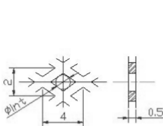
Filter 1/2" -> 2" Øint max = 1mm.
