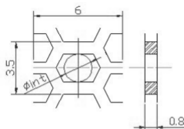
Filter 2 1/2" -> 4" Øint max = 1.9mm.
